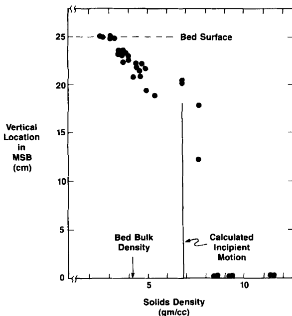
FIGURE 4: STRATIFICATION OF SOLIDS BY DENSITY IN A MAGNETICALLY STABILIZED FLUIDIZED BED
